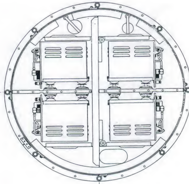
REAR VIEW OF CARTRIDGE WITH END PLATE REMOVED
